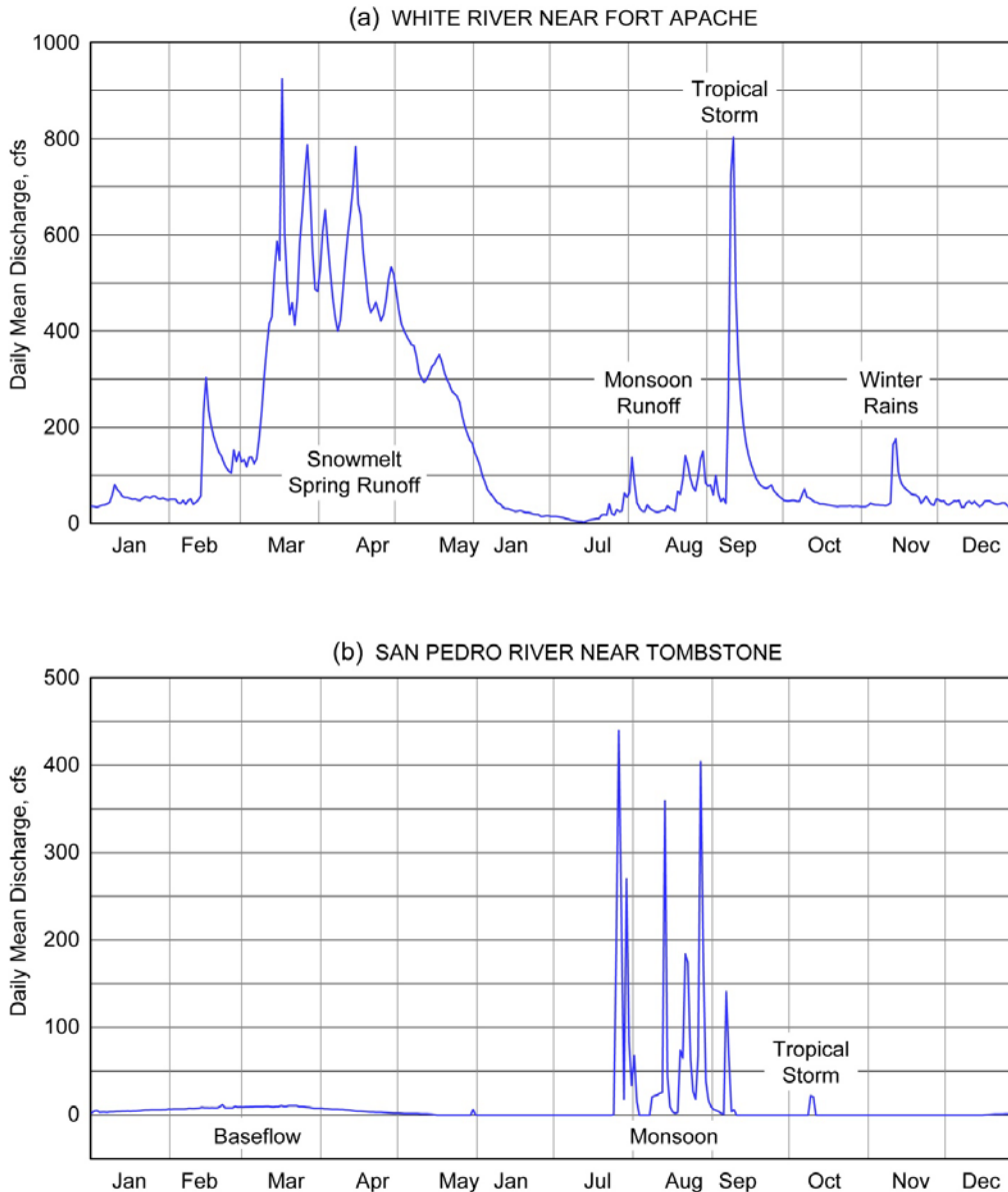
Figure 4-9. 2003 calendar year hydrographs from (a) the White River near Fort Apache, Arizona and (b) the San Pedro River near Tombstone, AZ.
