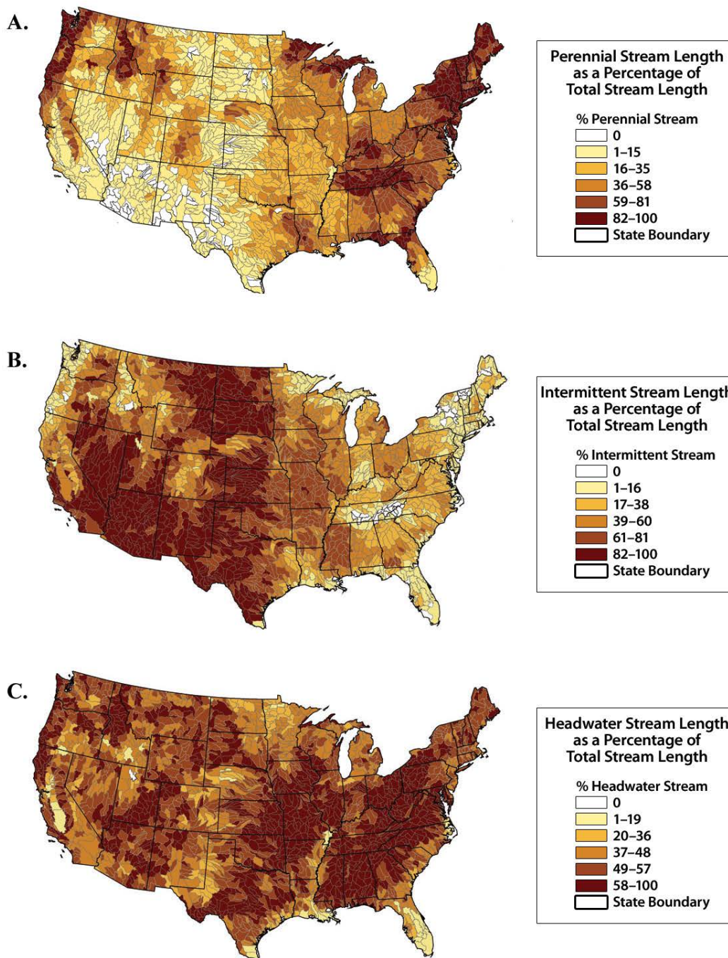
Figure 3-9. Characteristics of U.S. streams by watershed, in terms of percent of total stream length as (A) perennial, (B) intermittent, and (C) headwater streams. Data from the National Hydrographic Dataset (NHD) Reach Address Database (RAD) v2.0 at 1:100,000 scale using 8-digit HUC watersheds. Here, “intermittent” includes streams having intermittent or ephemeral flow. Note that NHD data generally do not capture streams <1.6 km, and ranges of color categories are not consistent across maps.
