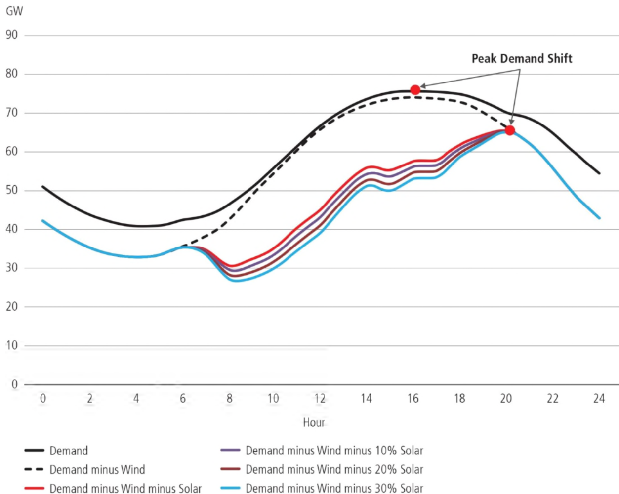
Figure 4.12. Demand and Net Demand Shapes at Different Distributed Energy Resource Penetration Levels 293
